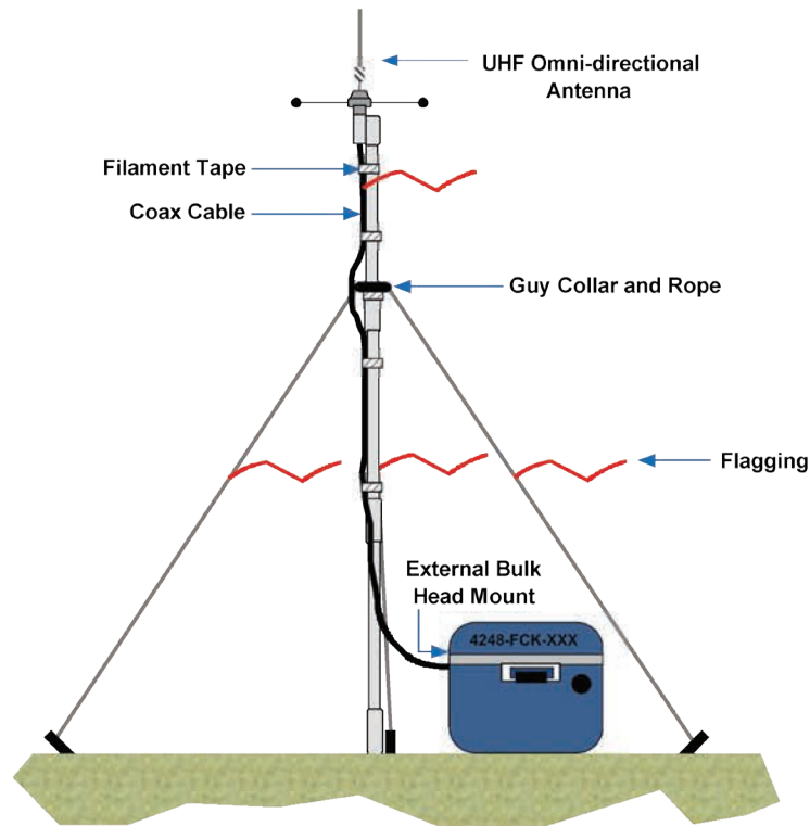
Figure 1: 4248 - UHF REPEATER ANTENNA SETUP
