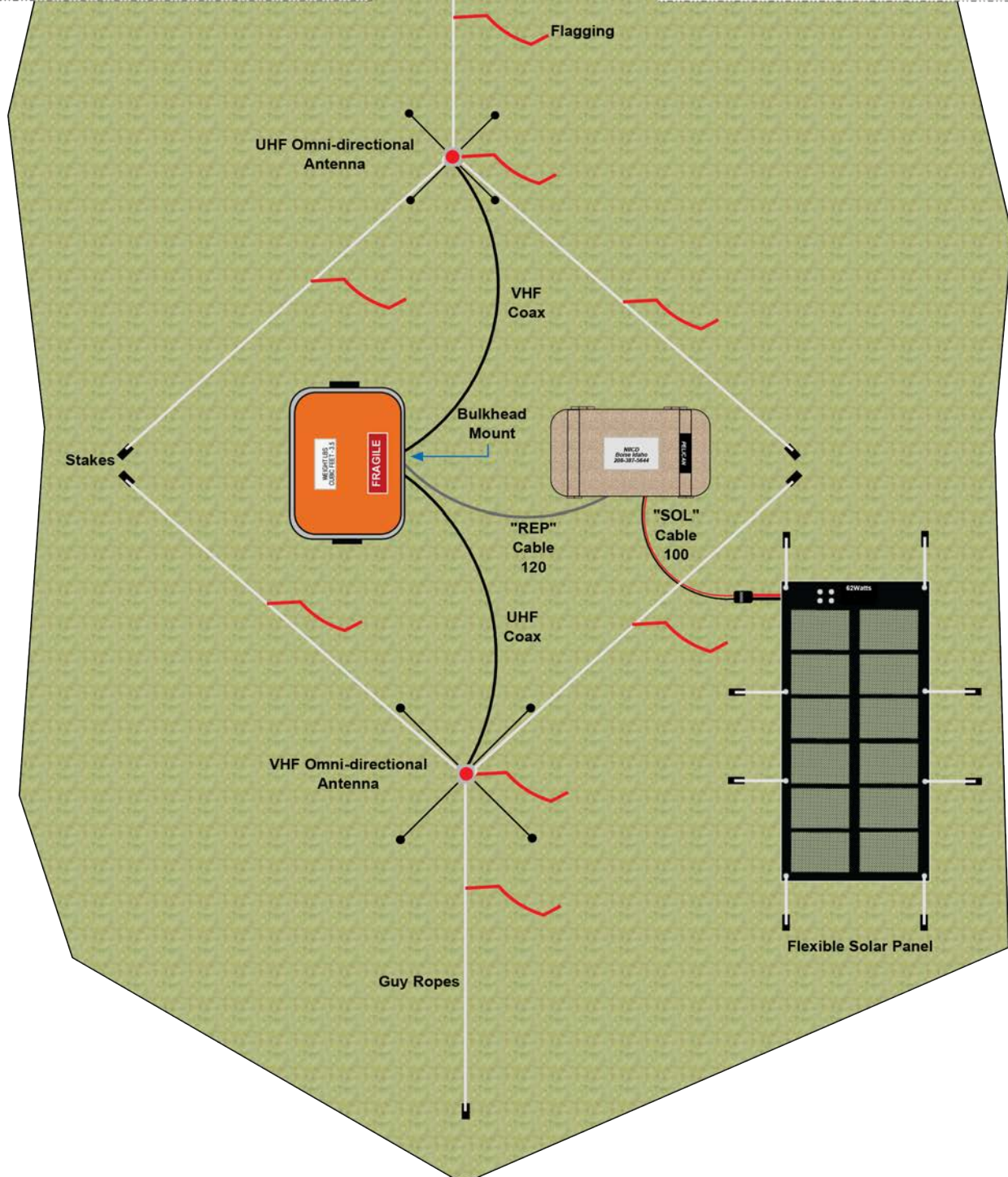
Figure 1: Solar Panel Installation (Overhead View)
