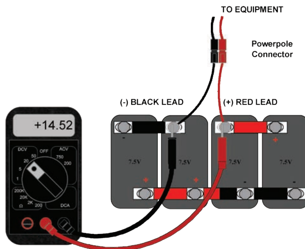
Figure 1: Sample Voltmeter Test with Equipment Under Transmit Load
