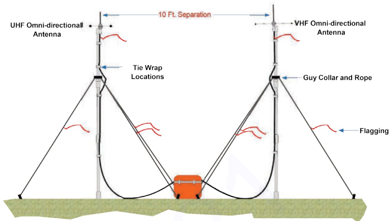
Figure 1: 4281 - CROSSBAND LINK ANTENNA SETUP
