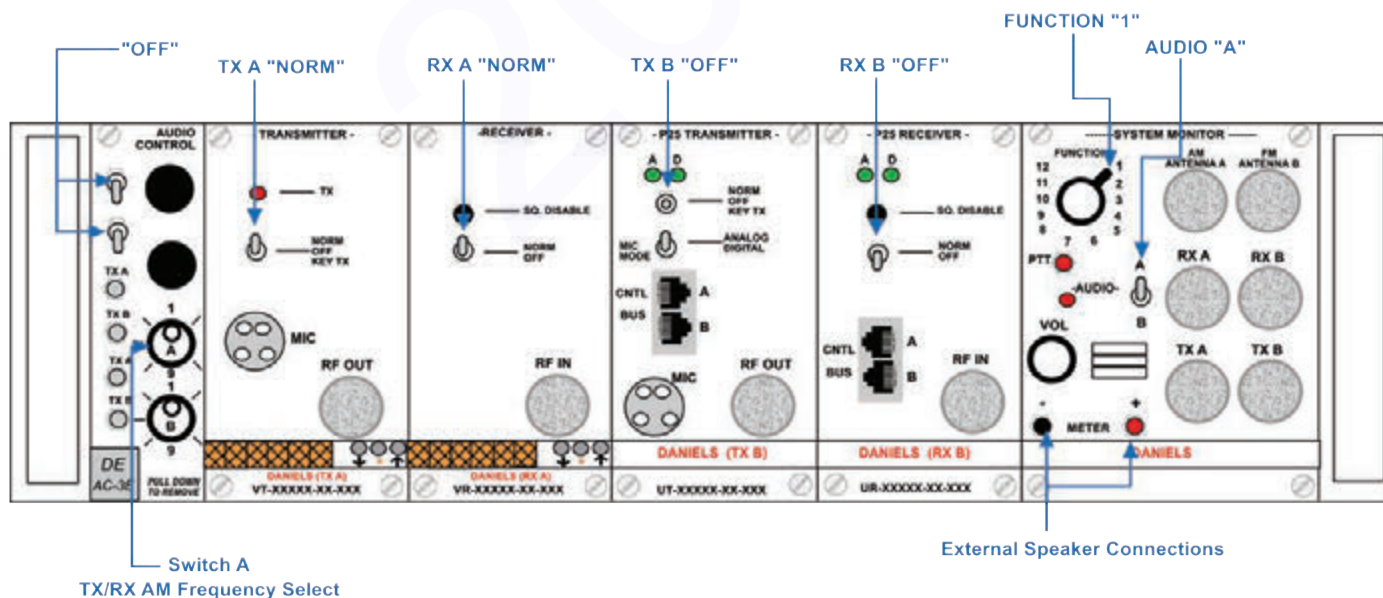
Figure 2: 4370 GROUND AIRCRAFT RADIO/LINK SWITCH SETTINGS BASE CONFIGURATION
