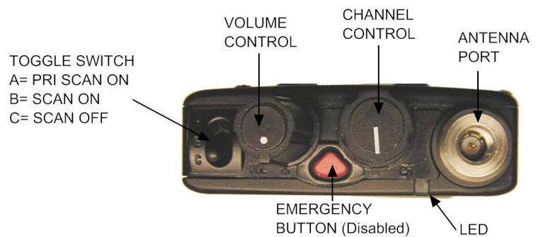
Figure 1: RACAL Top View
