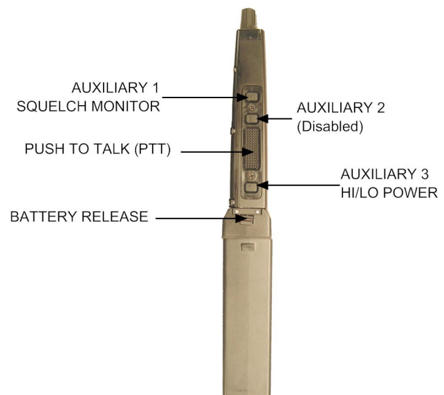
Figure 3: RACAL Side View
